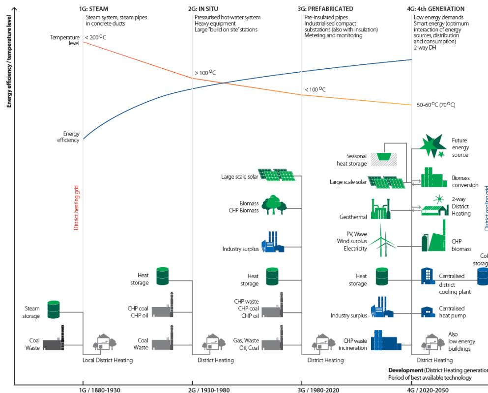
Figure 2. District heating generations by supply, efficiency, and temperature level
